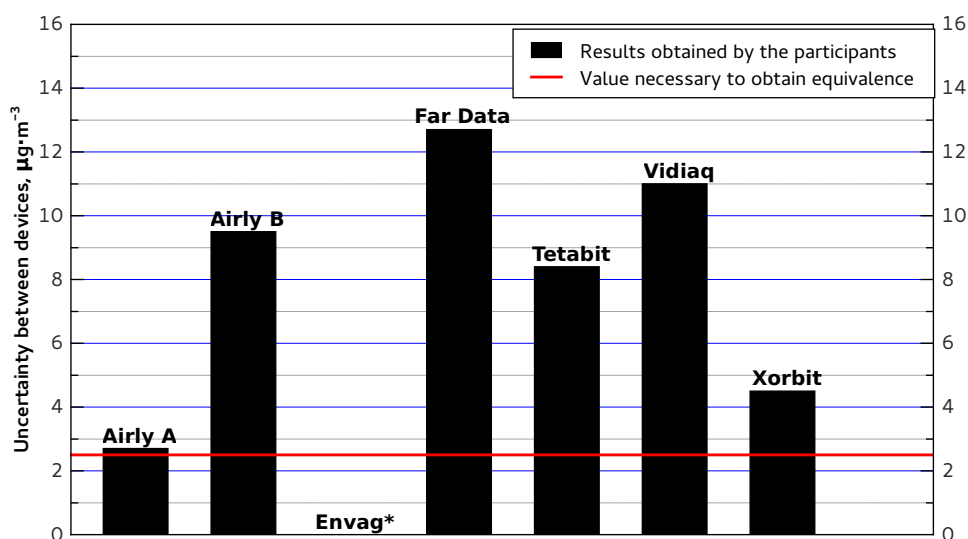
Figure 3.6: II series of measurements: uncertainty of average daily indications of PM 2.5 concentration between two devices held by a given participant in the entire period analysed excluding average daily values below 30 \mu\text{g}/\text{m}^3 . The red line marks the level that cannot be crossed by the devices which are to be recognised as equivalent. The Warsaw University of Technology was not included in this comparison due to the lack of results for PM 2.5 obtained with the use of this participant's devices. *) The "0" value for the company Envag results from the fact that this participant's devices did not report the values above 30 \mu\text{g}/\text{m}^3 . Prepared on the basis of the report [2].
