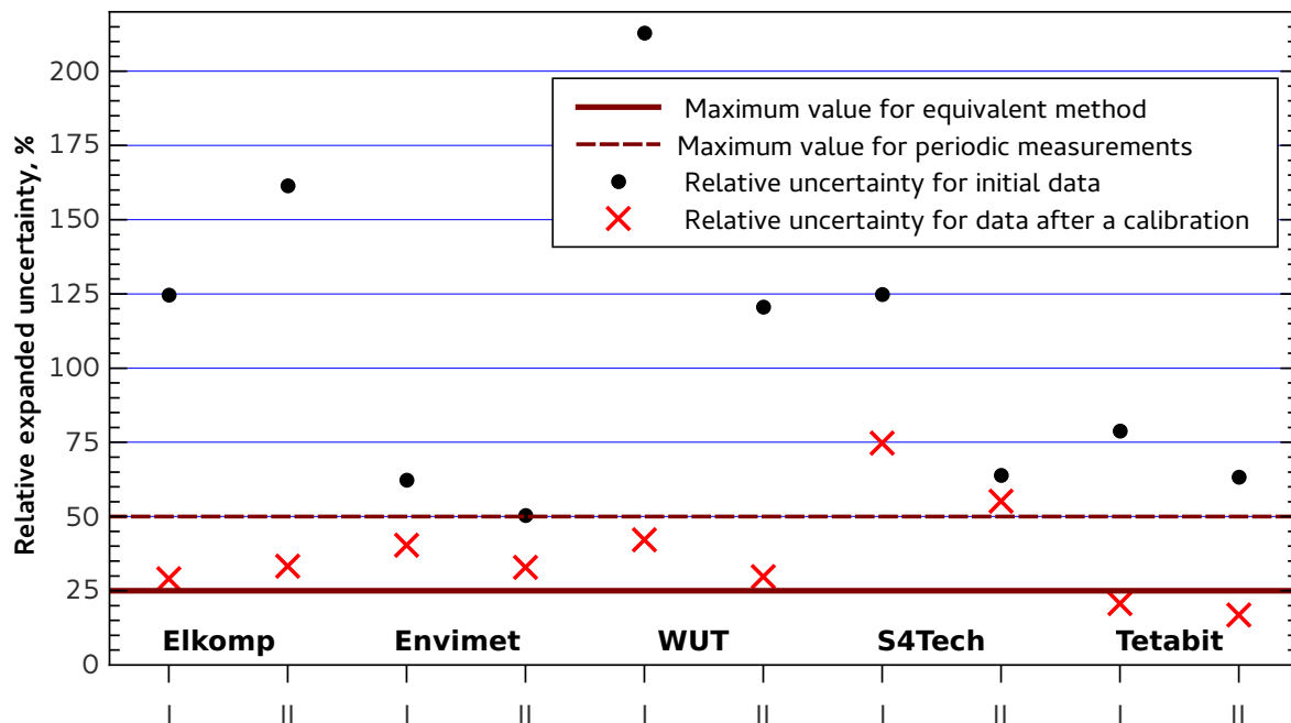
Figure 3.10: I Edycja: relative expanded uncertainty of the PM 10 daily average concentration measurement for particular devices before and after a calibration. Prepared on the basis of the report [1].
