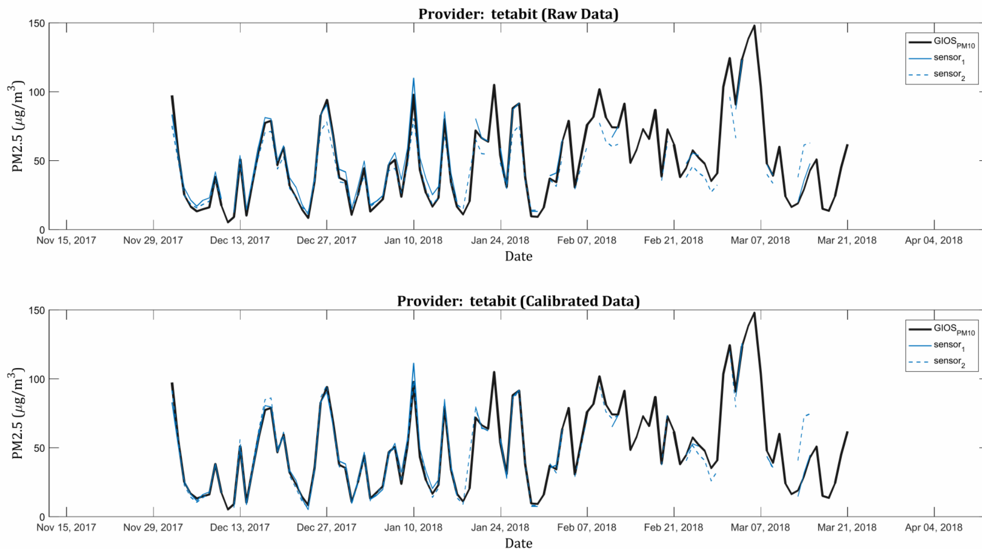
Figure C.13: Comparison of the results of the PM2.5 average daily concentration measurements for the sensors produced by Tetabit (blue lines) with the values provided by the National Reference and Calibration Laboratory of the Chief Inspectorate for Environmental Protection (black line). The first chart presents the data provided by the participants. The lower chart presents the data after a recalibration has been conducted by the report authors [2].
