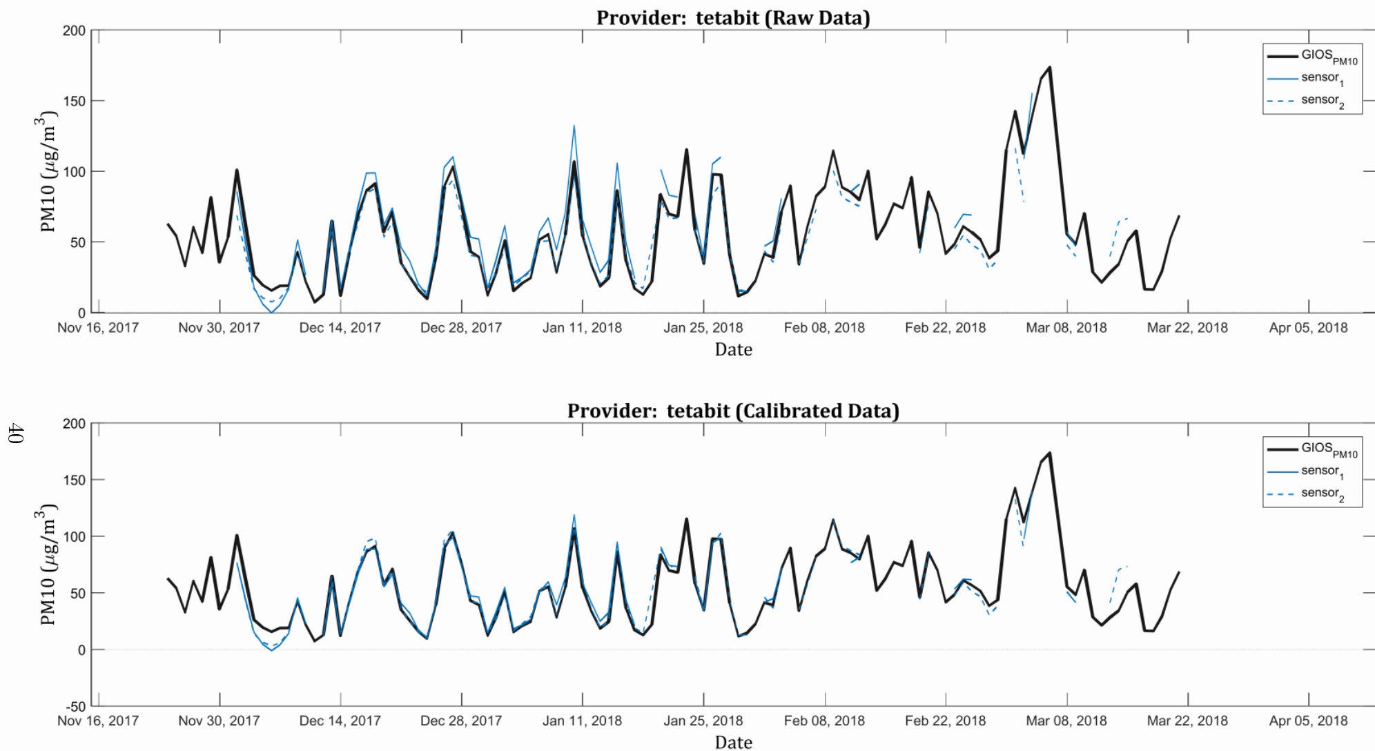
Figure C.6: Comparison of the results of the PM10 average daily concentration measurements for the sensors produced by Tetabit (blue lines) with the values provided by the National Reference and Calibration Laboratory of the Chief Inspectorate for Environmental Protection (black line). The first chart presents the data provided by the participants. The lower chart presents the data after a recalibration has been conducted by the report authors [2].
