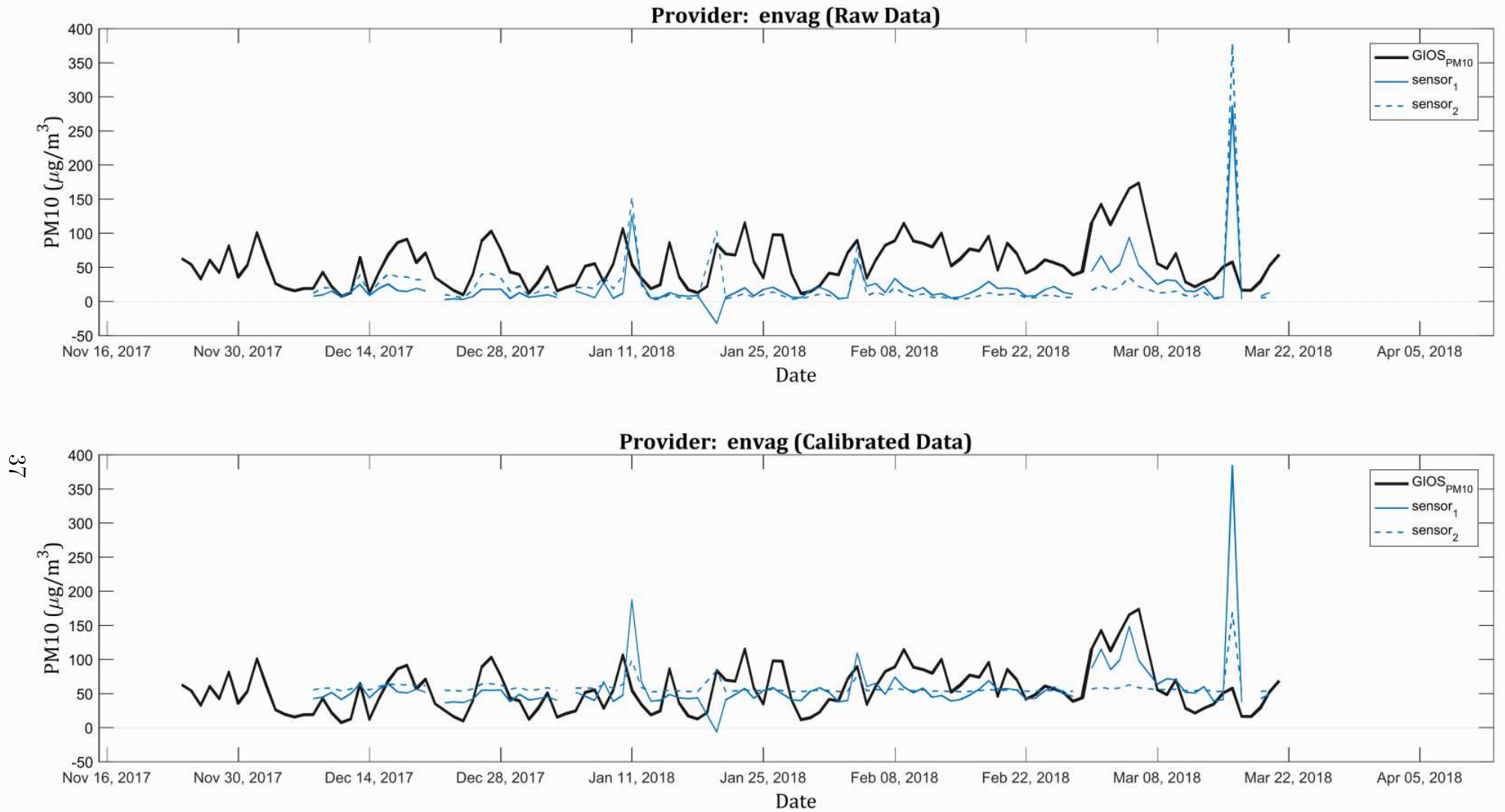
Figure C.3: Comparison of the results of the PM10 average daily concentration measurements for the sensors produced by Envag (blue lines) with the values provided by the National Reference and Calibration Laboratory of the Chief Inspectorate for Environmental Protection (black line). The first chart presents the data provided by the participants. The lower chart presents the data after a recalibration has been conducted by the report authors [2].
