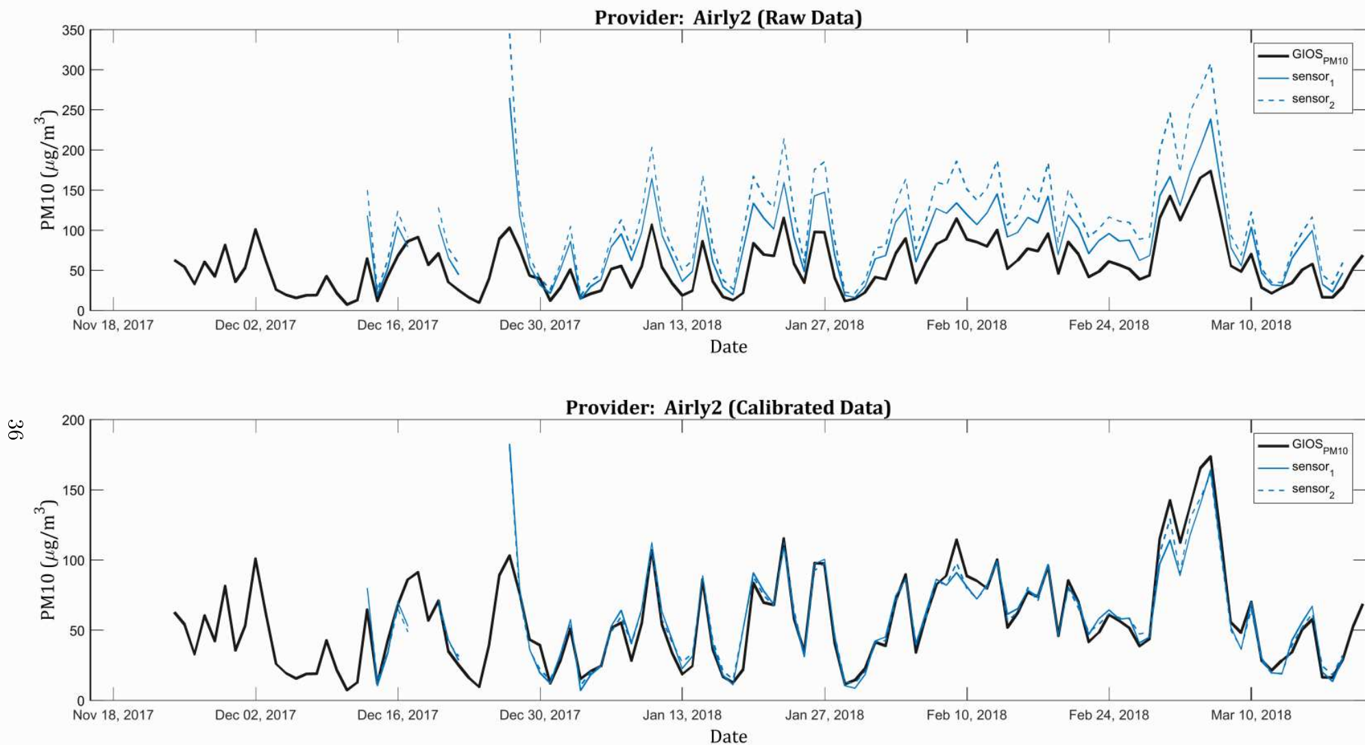
Figure C.2: Comparison of the results of the PM10 average daily concentration measurements for the sensors produced by Airly set B (blue lines) with the values provided by the National Reference and Calibration Laboratory of the Chief Inspectorate for Environmental Protection (black line). The first chart presents the data provided by the participants. The lower chart presents the data after a recalibration has been conducted by the report authors [2].
