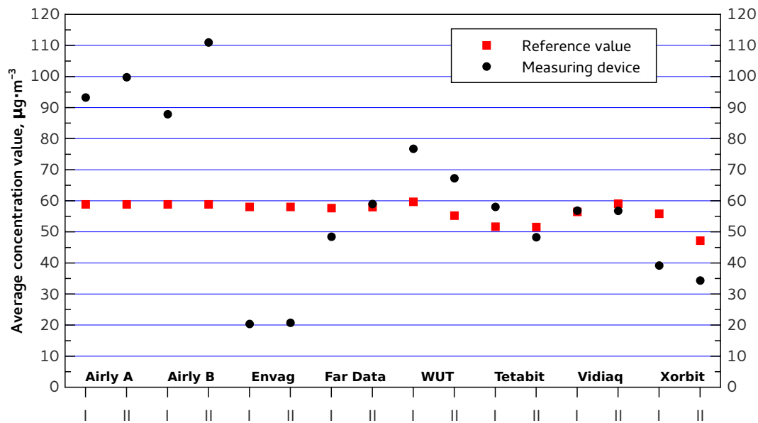
Figure 3.8: II series of measurements: comparison of the PM10 average concentration values obtained with the use of the tested devices with a reference method. The average values were calculated for each device before a calibration and compared with the average value obtained in the period in which the device reported data. Prepared on the basis of the report [2].
