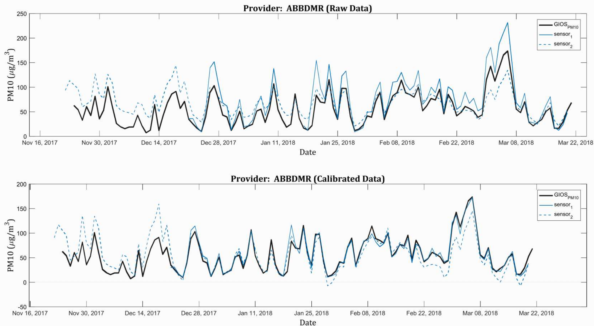
Figure C.5: Comparison of the results of the PM10 average daily concentration measurements for the sensors produced by Warsaw University of Technology (blue lines) with the values provided by the National Reference and Calibration Laboratory of the Chief Inspectorate for Environmental Protection (black line). The first chart presents the data provided by the participants. The lower chart presents the data after a recalibration has been conducted by the report authors [2].
