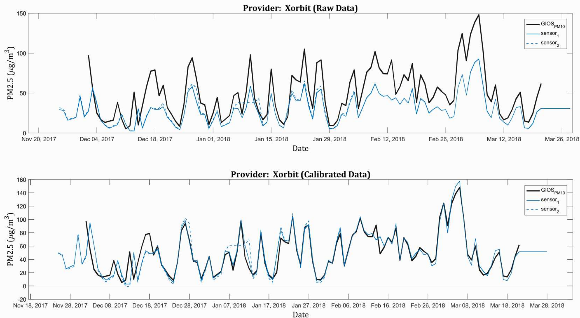
Figure C.15: Comparison of the results of the PM2.5 average daily concentration measurements for the sensors produced by Xorbit (blue lines) with the values provided by the National Reference and Calibration Laboratory of the Chief Inspectorate for Environmental Protection (black line). The first chart presents the data provided by the participants. The lower chart presents the data after a recalibration has been conducted by the report authors [2].
