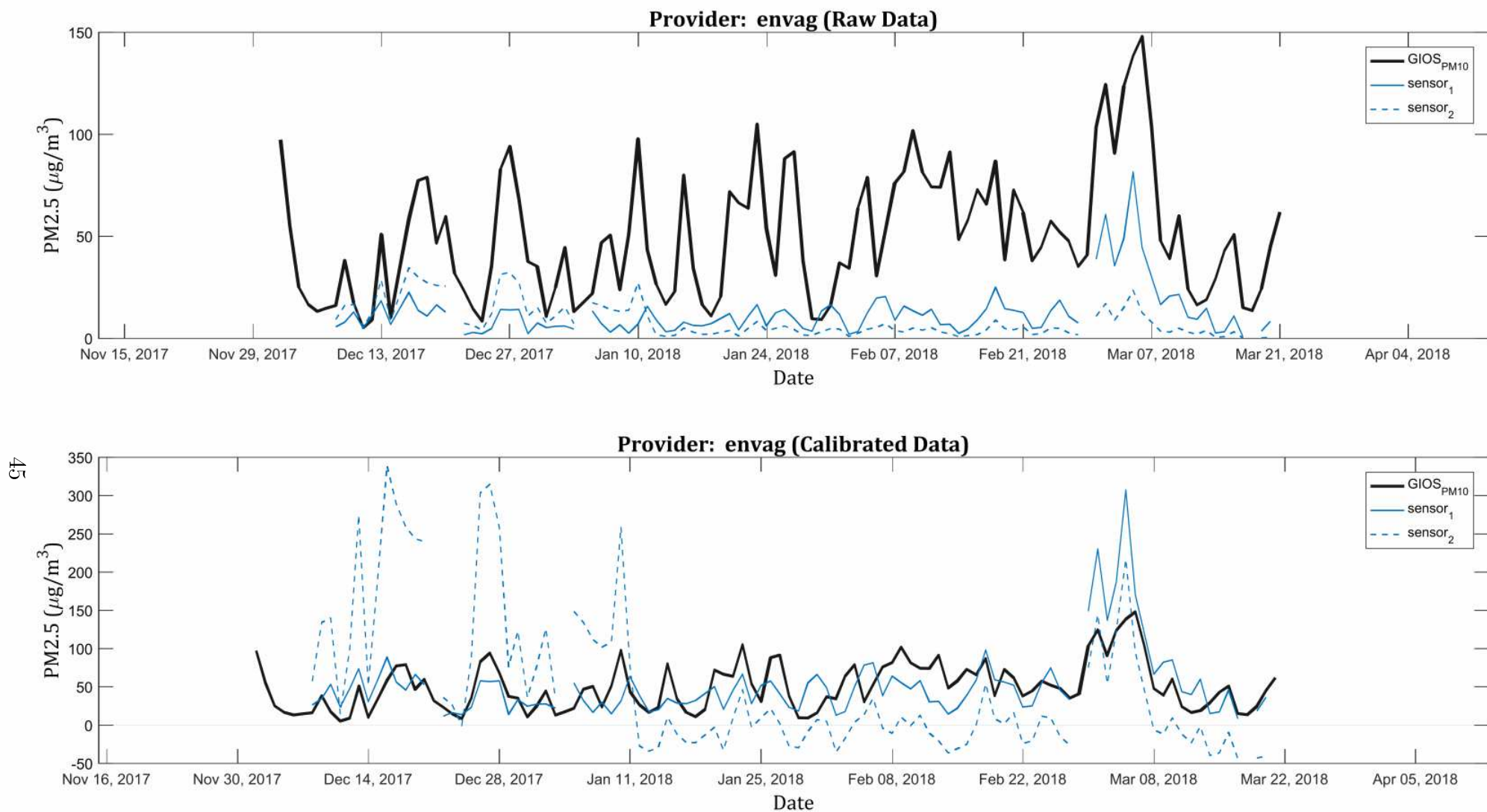
Figure C.11: Comparison of the results of the PM2.5 average daily concentration measurements for the sensors produced by Envag (blue lines) with the values provided by the National Reference and Calibration Laboratory of the Chief Inspectorate for Environmental Protection (black line). The first chart presents the data provided by the participants. The lower chart presents the data after a recalibration has been conducted by the report authors [2].
