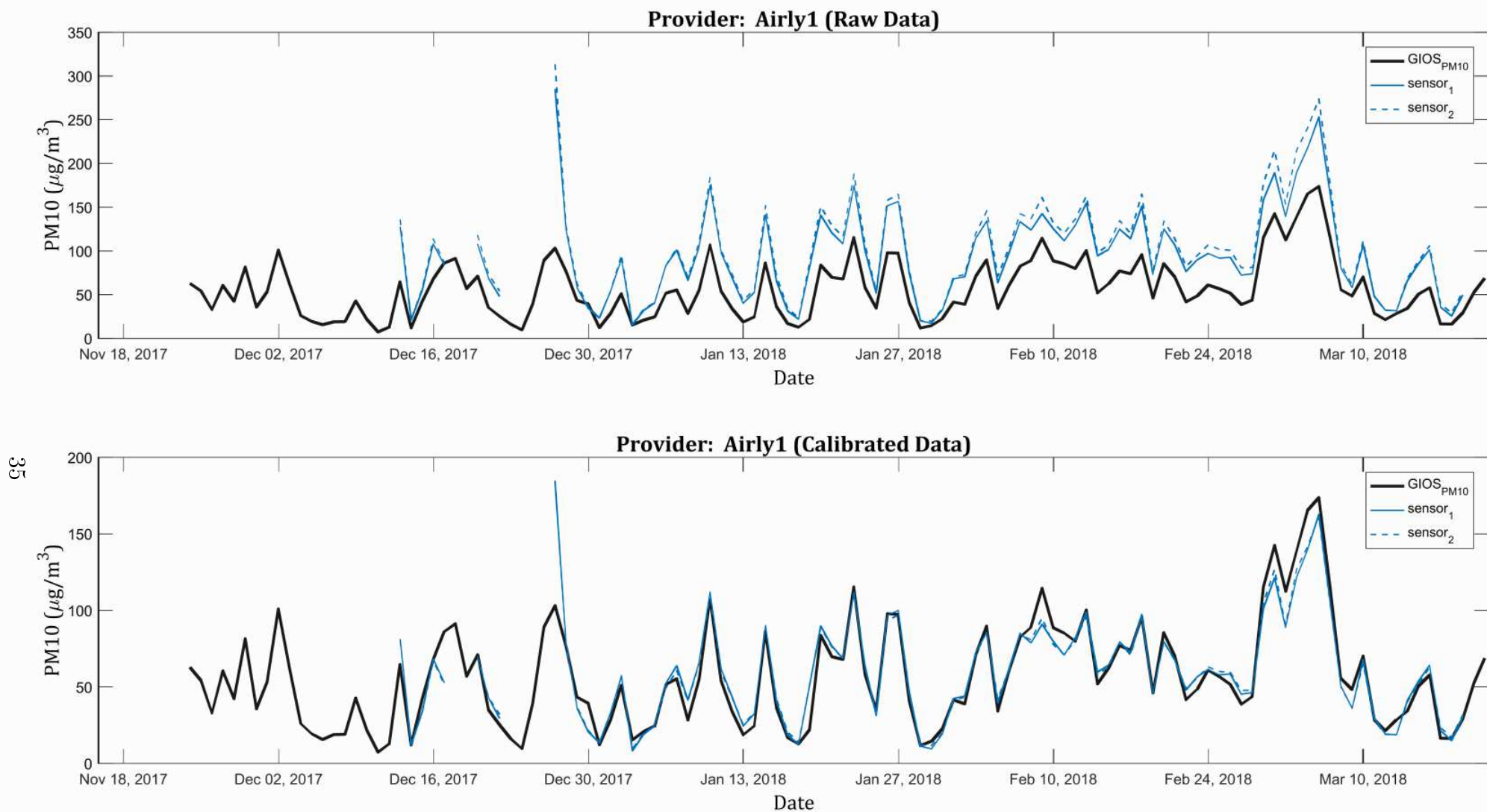
Figure C.1: Comparison of the results of the PM10 average daily concentration measurements for the sensors produced by Airly set A (blue lines) with the values provided by the National Reference and Calibration Laboratory of the Chief Inspectorate for Environmental Protection (black line). The first chart presents the data provided by the participants. The lower chart presents the data after a recalibration has been conducted by the report authors [2].
