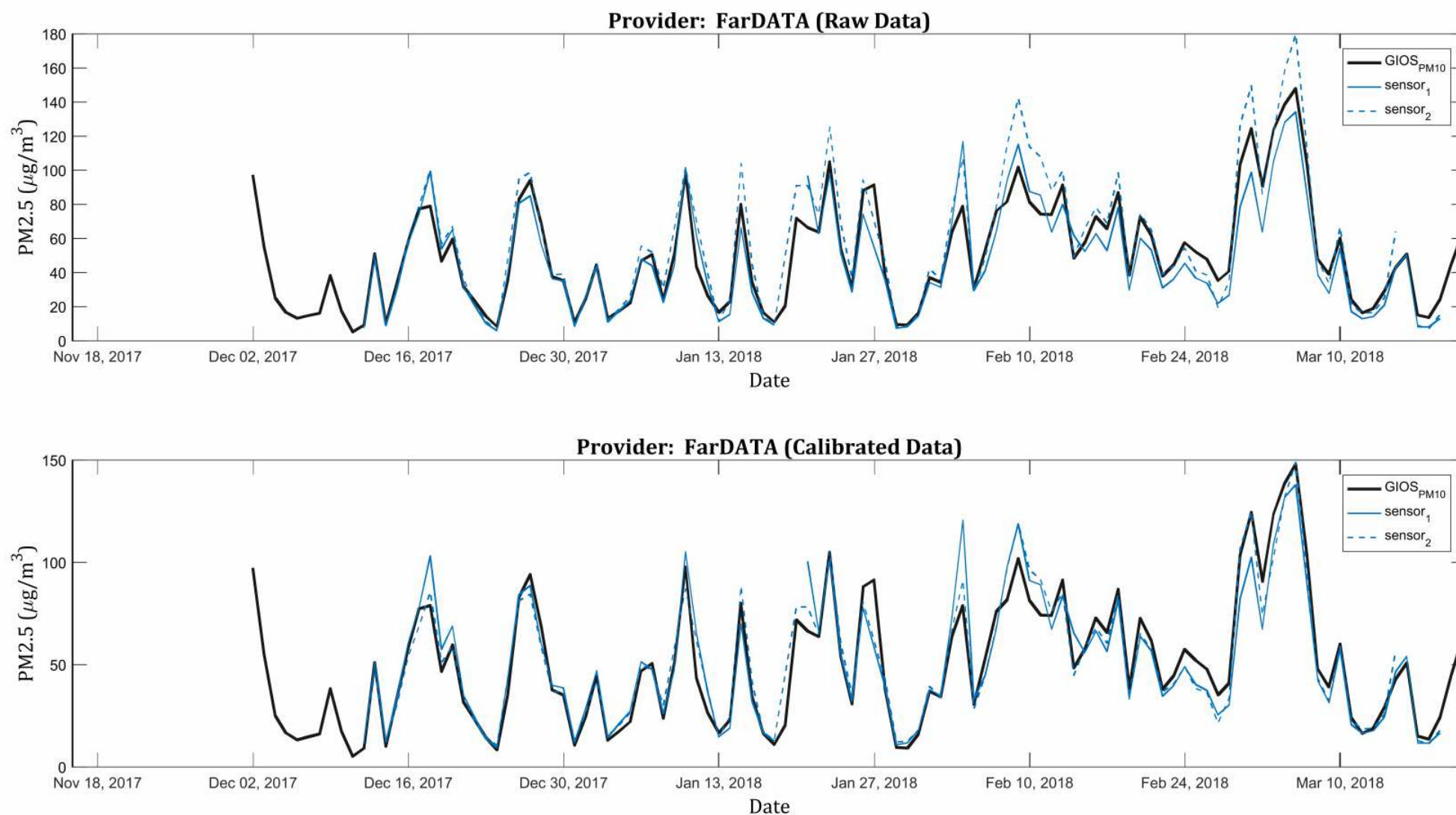
Figure C.12: Comparison of the results of the PM 2.5 average daily concentration measurements for the sensors produced by Far Data (blue lines) with the values provided by the National Reference and Calibration Laboratory of the Chief Inspectorate for Environmental Protection (black line). The first chart presents the data provided by the participants. The lower chart presents the data after a recalibration has been conducted by the report authors [2].
