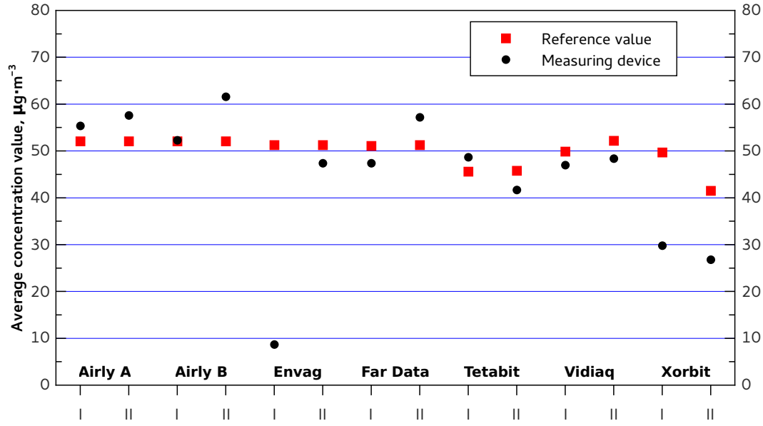
Figure 3.9: II series of measurements: comparison of the PM2.5 average concentration values obtained with the use of the tested devices with a reference method. The average values were calculated for each device before a calibration and compared with the average value obtained in the period in which the device reported data. Prepared on the basis of the report [2].
