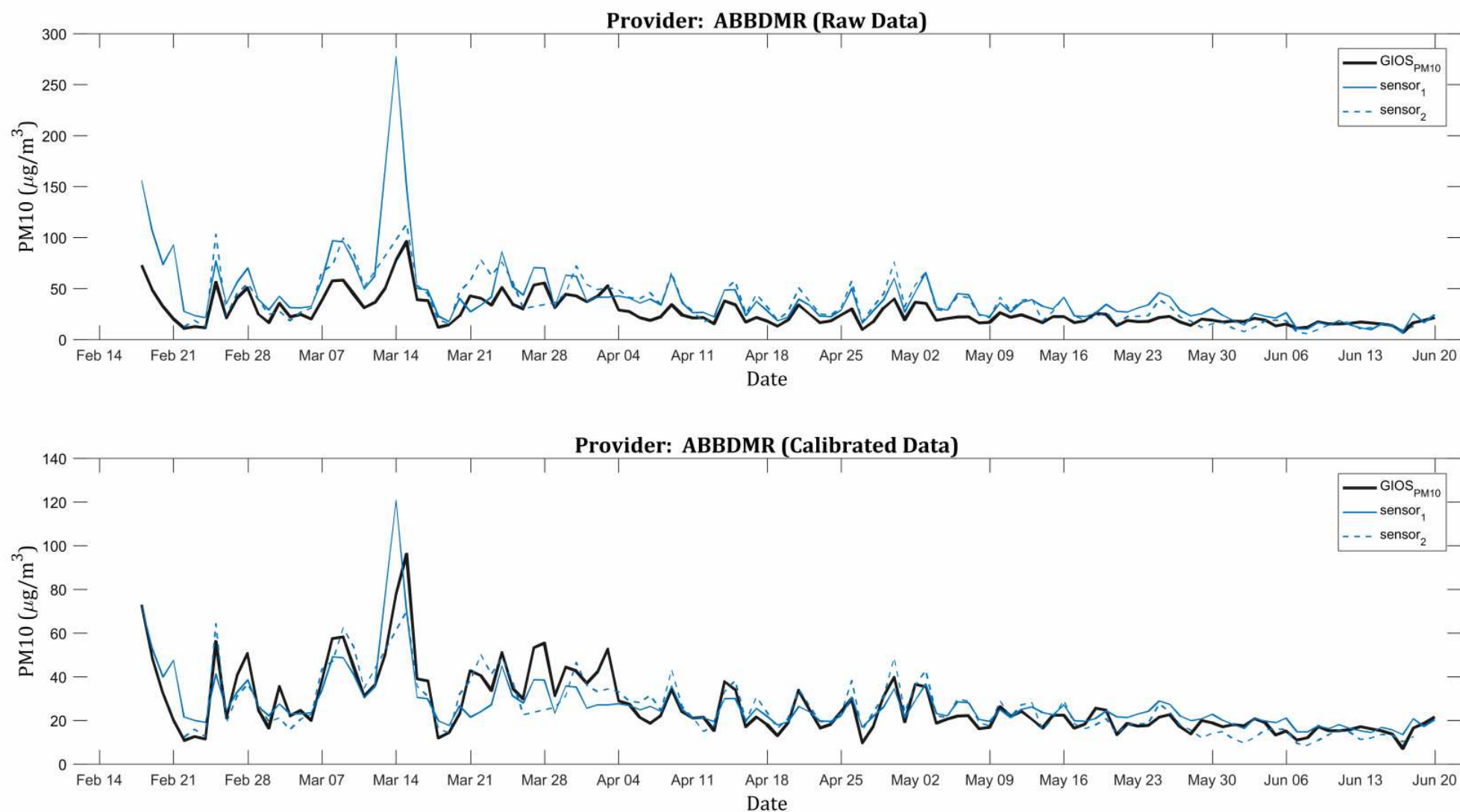
Figure B.3: Comparison of the results of the PM10 average daily concentration measurements for the sensors produced by Warsaw University of Technology (blue lines) with the values provided by the National Reference and Calibration Laboratory of the Chief Inspectorate for Environmental Protection (black line). The first chart presents the data provided by the participants. The lower chart presents the data after a recalibration has been conducted by the report authors [1].
