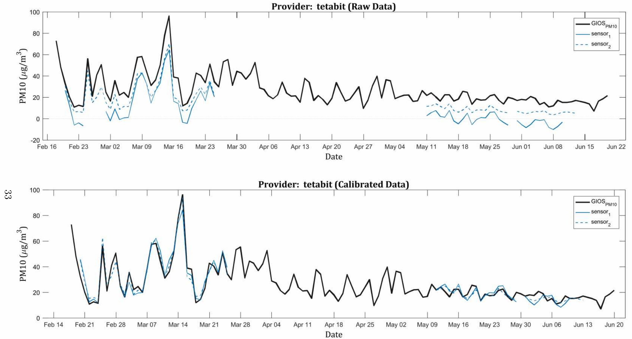
Figure B.5: Comparison of the results of the PM10 average daily concentration measurements for the sensors produced by Tetabit (blue lines) with the values provided by the National Reference and Calibration Laboratory of the Chief Inspectorate for Environmental Protection (black line). The first chart presents the data provided by the participants. The lower chart presents the data after a recalibration has been conducted by the report authors [1].
