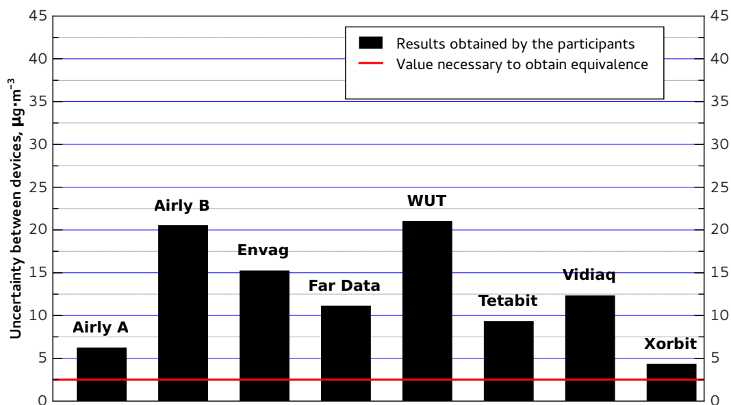
Figure 3.2: I series of measurements: uncertainty of average daily indications of PM10 concentration between two devices held by a given participant in the entire period analysed excluding average daily values below \mu\text{g}/\text{m}^3 . The red line marks the level that cannot be crossed by the devices which are to be recognised as equivalent. Prepared on the basis of the report [1].
