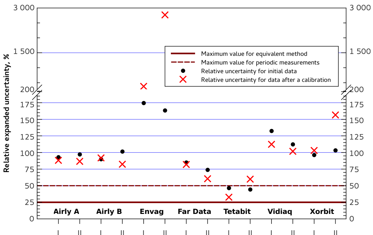
Figure 3.12: II Edycja: relative expanded uncertainty of the PM2.5 daily average concentration measurement for particular devices before and after a calibration. Due to considerable differences between the participants, intercepts and various scales were used for a chart divided in this way. Prepared on the basis of the report [2].
