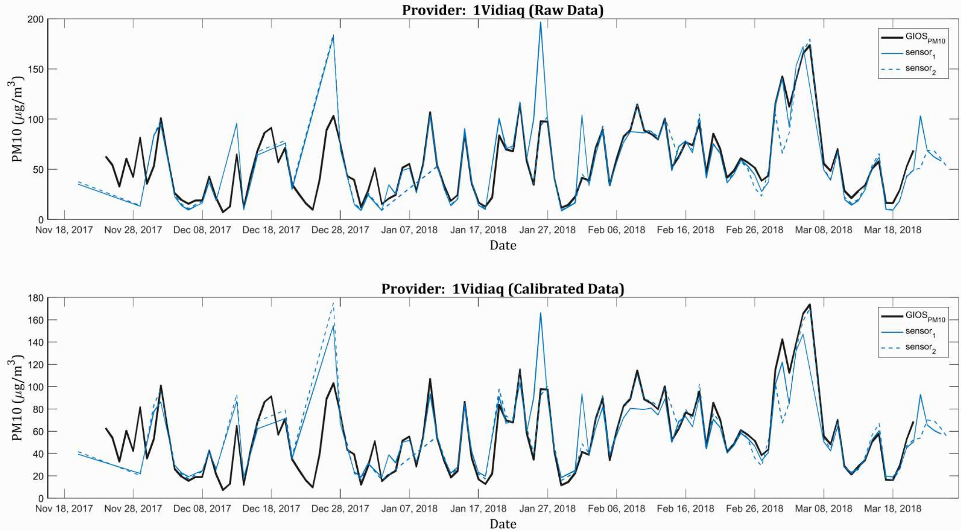
Figure C.7: Comparison of the results of the PM10 average daily concentration measurements for the sensors produced by Vidiaq (blue lines) with the values provided by the National Reference and Calibration Laboratory of the Chief Inspectorate for Environmental Protection (black line). The first chart presents the data provided by the participants. The lower chart presents the data after a recalibration has been conducted by the report authors [2].
