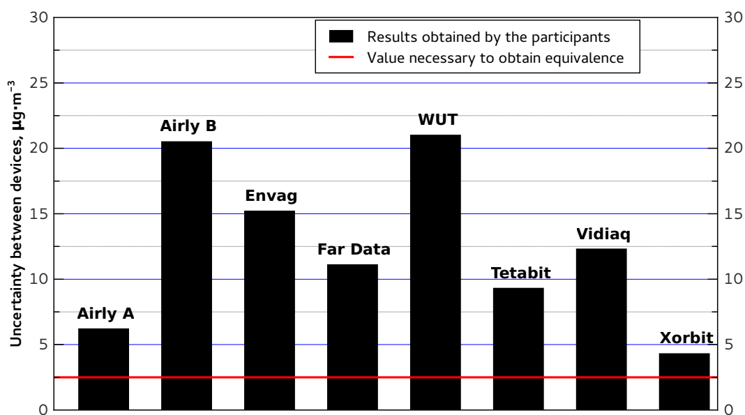
Figure 3.3: II series of measurements: uncertainty of average daily indications of PM10 concentration between two devices held by a given participant in the entire period analysed. The red line marks the level that cannot be crossed by the devices which are to be recognised as equivalent. Prepared on the basis of the report [2].
