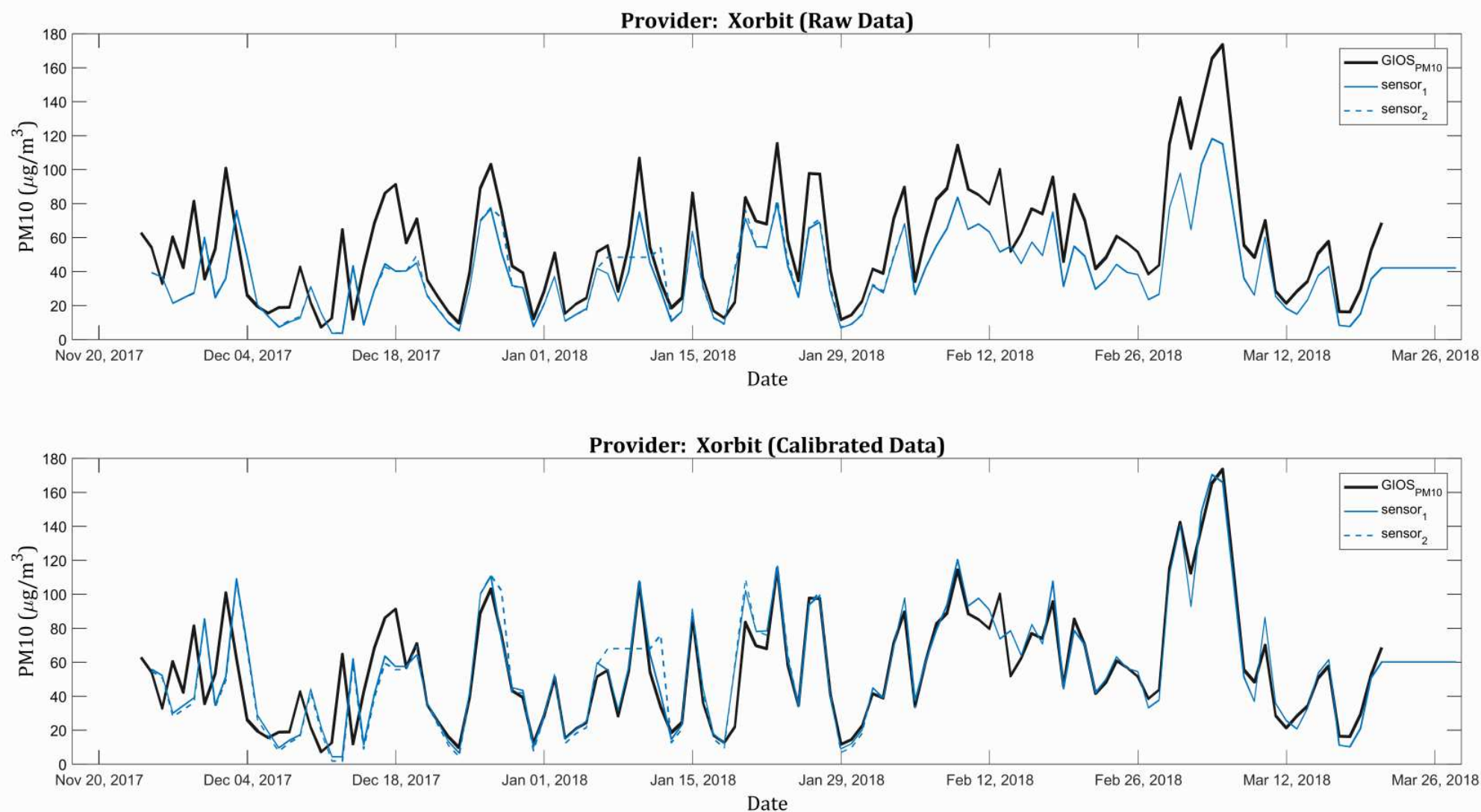
Figure C.8: Comparison of the results of the PM10 average daily concentration measurements for the sensors produced by Xorbit (blue lines) with the values provided by the National Reference and Calibration Laboratory of the Chief Inspectorate for Environmental Protection (black line). The first chart presents the data provided by the participants. The lower chart presents the data after a recalibration has been conducted by the report authors [2].
