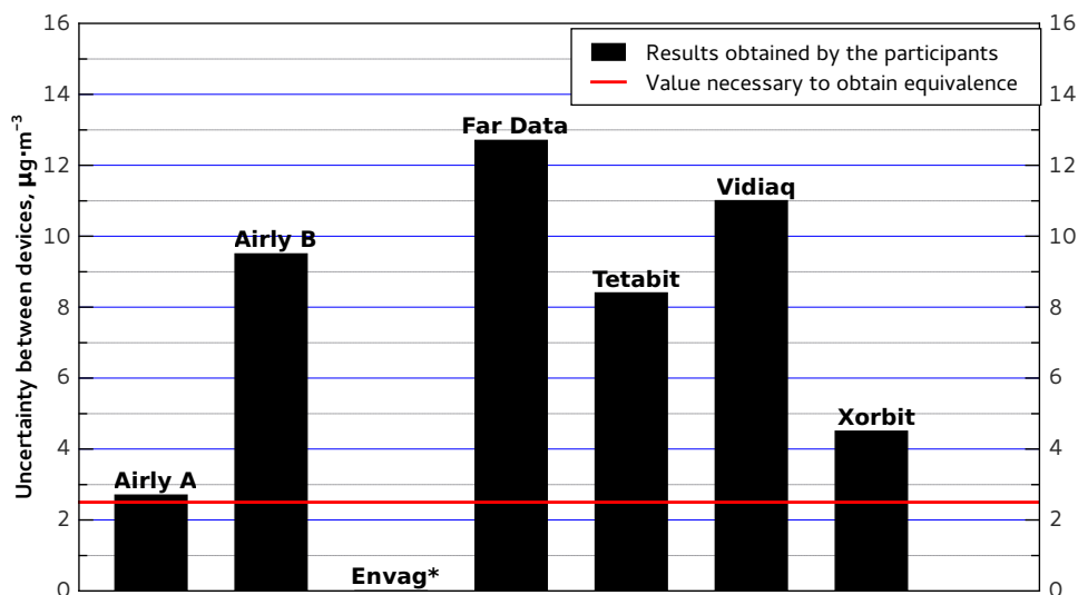
Figure 3.5: II series of measurements: uncertainty of average daily indications of PM 2.5 concentration between two devices held by a given participant in the entire period analysed. The red line marks the level that cannot be crossed by the devices which are to be recognised as equivalent. The Warsaw University of Technology was not included in this comparison due to the lack of results for PM 2.5 obtained with the use of this participant's devices. Prepared on the basis of the report [2].
