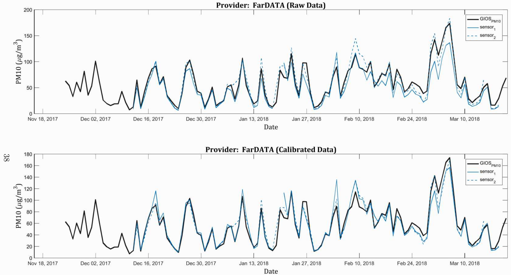
Figure C.4: Comparison of the results of the PM10 average daily concentration measurements for the sensors produced by Far Data (blue lines) with the values provided by the National Reference and Calibration Laboratory of the Chief Inspectorate for Environmental Protection (black line). The first chart presents the data provided by the participants. The lower chart presents the data after a recalibration has been conducted by the report authors [2].
