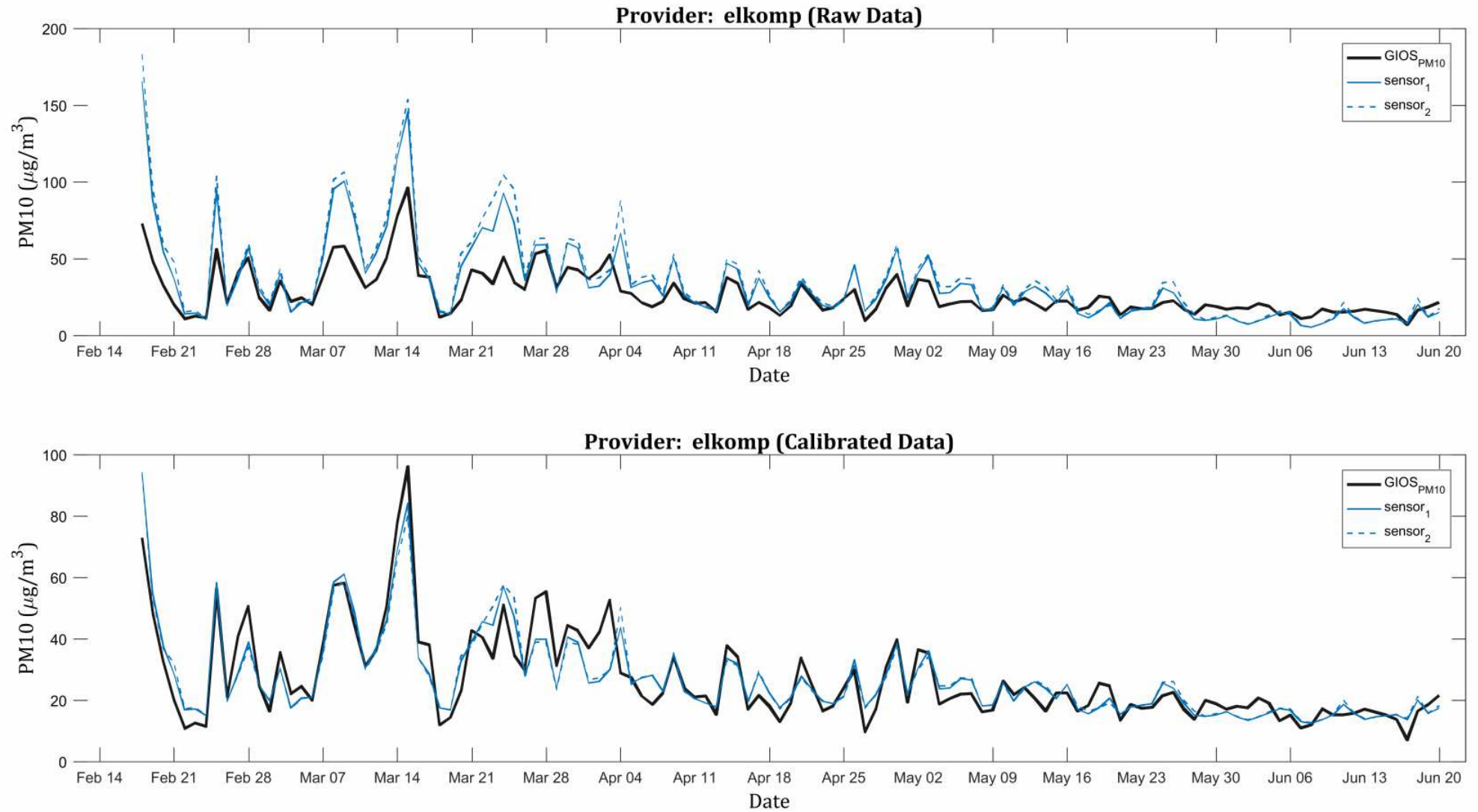
Figure B.1: Comparison of the results of the PM10 average daily concentration measurements for the sensors produced by Elkomp (blue lines) with the values provided by the National Reference and Calibration Laboratory of the Chief Inspectorate for Environmental Protection (black line). The first chart presents the data provided by the participants. The lower chart presents the data after a recalibration has been conducted by the report authors [1].
