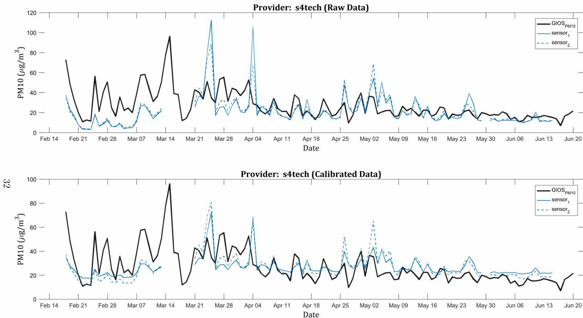
Figure B.4: Comparison of the results of the PM10 average daily concentration measurements for the sensors produced by S4Tech (blue lines) with the values provided by the National Reference and Calibration Laboratory of the Chief Inspectorate for Environmental Protection (black line). The first chart presents the data provided by the participants. The lower chart presents the data after a recalibration has been conducted by the report authors [1].
