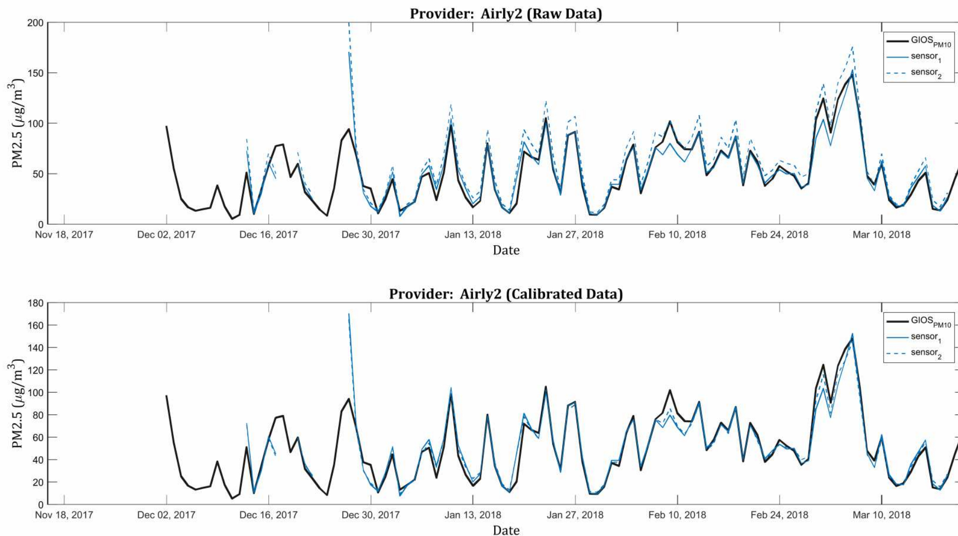
Figure C.10: Comparison of the results of the PM2.5 average daily concentration measurements for the sensors produced by Airly set B (blue lines) with the values provided by the National Reference and Calibration Laboratory of the Chief Inspectorate for Environmental Protection (black line). The first chart presents the data provided by the participants. The lower chart presents the data after a recalibration has been conducted by the report authors [2].
