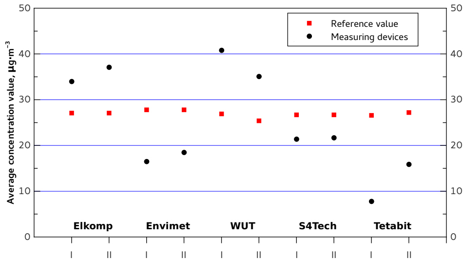
Figure 3.7: I series of measurements: comparison of the PM10 average concentration values obtained with the use of the tested devices with a reference method. The average values were calculated for each device before a calibration and compared with the average value obtained in the period in which the device reported data. Prepared on the basis of the report [1].
