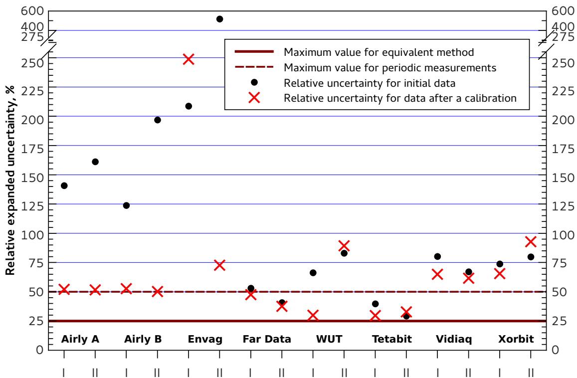
Figure 3.11: II Edycja: relative expanded uncertainty of the PM10 daily average concentration measurement for particular devices before and after a calibration. Due to considerable differences between the participants, intercepts and various scales were used for a chart divided in this way. Prepared on the basis of the report [2].
