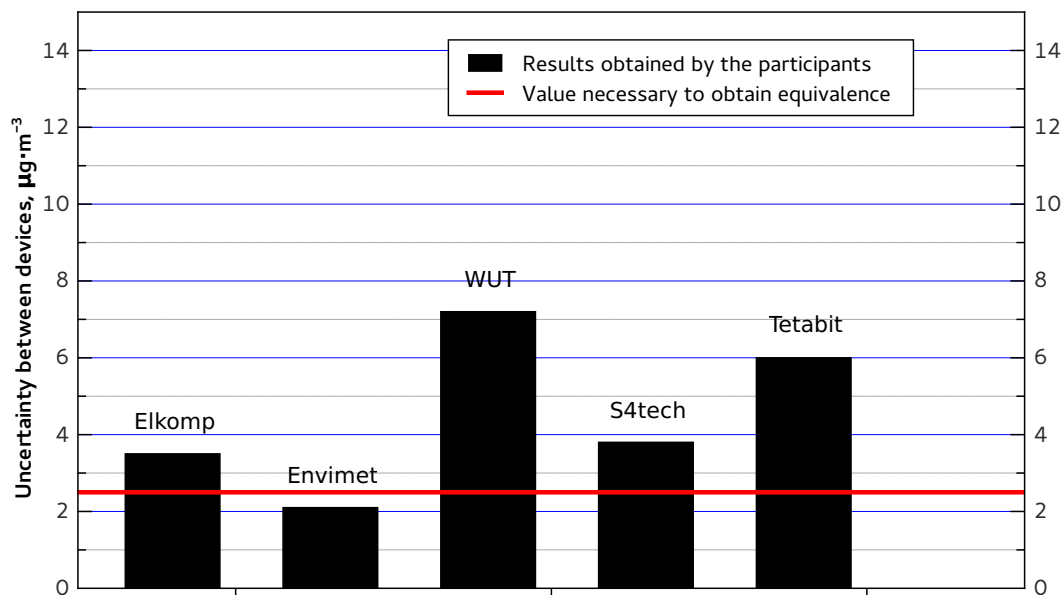
Figure 3.1: I series of measurements: uncertainty of average daily indications of PM10 concentration between two devices held by a given participant in the entire period analysed. The red line marks the level that cannot be crossed by the devices which are to be recognised as equivalent. Prepared on the basis of the report [1].
