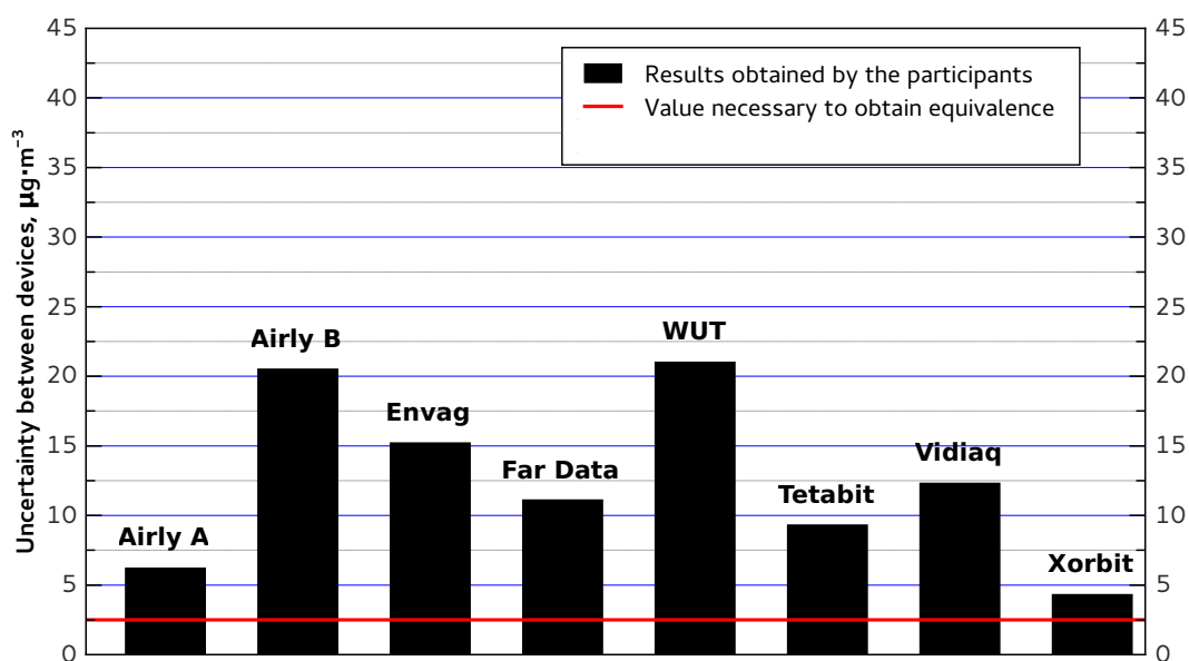
Figure 3.4: II series of measurements: uncertainty of average daily indications of PM10 concentration between two devices held by a given participant in the entire period analysed excluding average daily values below 30 \mu\text{g}/\text{m}^3 . The red line marks the level that cannot be crossed by the devices which are to be recognised as equivalent. Prepared on the basis of the report [2].
