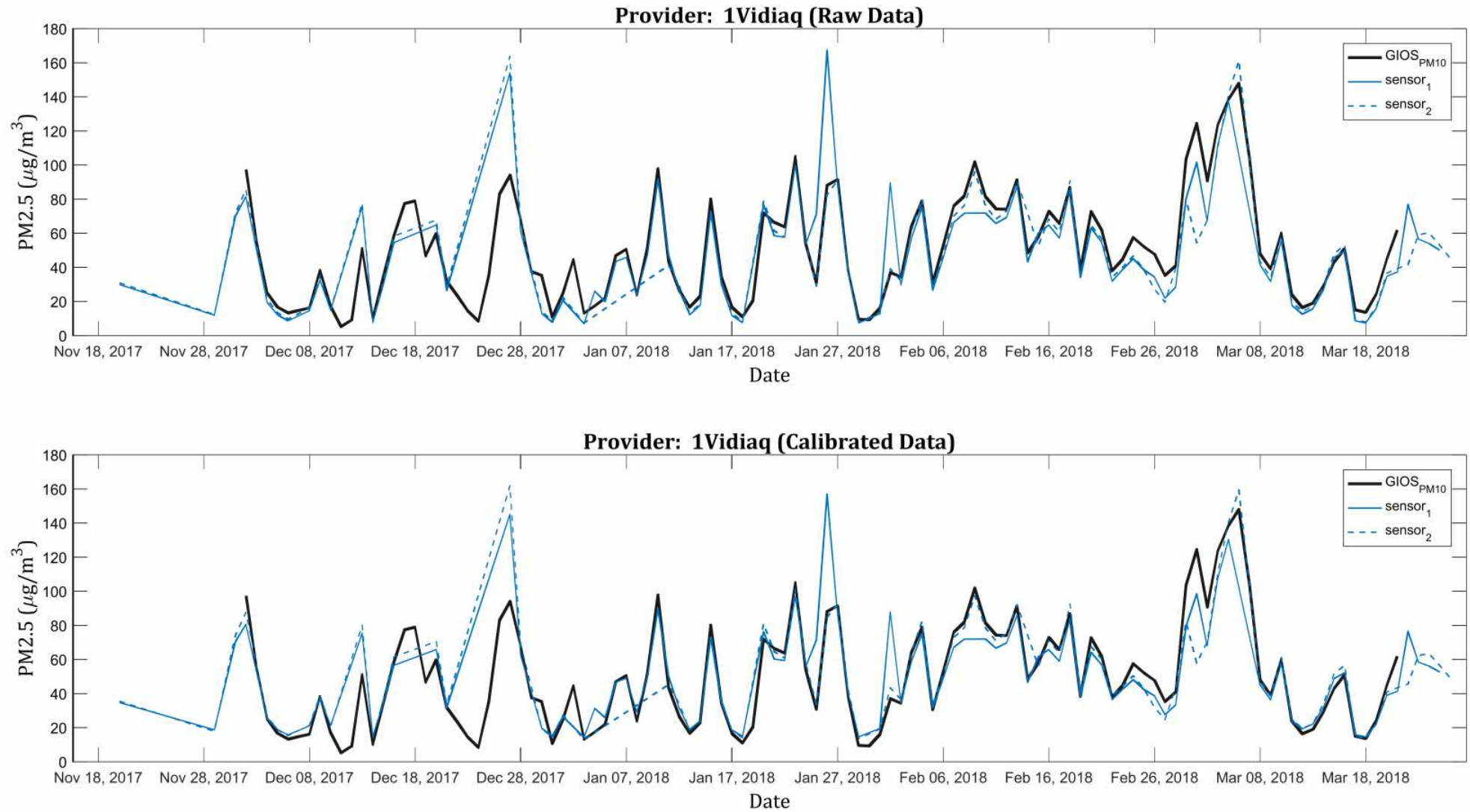
Figure C.14: Comparison of the results of the PM 2.5 average daily concentration measurements for the sensors produced by Vidiaq (blue lines) with the values provided by the National Reference and Calibration Laboratory of the Chief Inspectorate for Environmental Protection (black line). The first chart presents the data provided by the participants. The lower chart presents the data after a recalibration has been conducted by the report authors [2].
